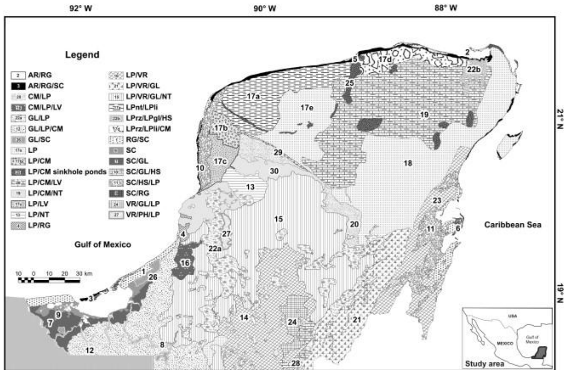
Figure 4: Soilscapes of the Yucatan considering geomorphology and soils. LP = Leptosols, CM = Cambisols, VR = Vertisols, GL = Gleysols, SC = Solonchak, RG = Regosols, AR = Arenosols, NT = Nitisols, PH = Pheozems, HS = Histosols, nt = Nudilithic, li = lithic, rz = Rendzic, and gl = gleyic (Bautista et al. 2011: Fig. 5)
