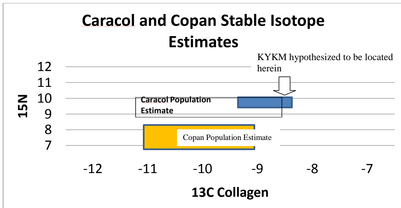
Figure 5. Caracol and Copan stable isotope maps.
